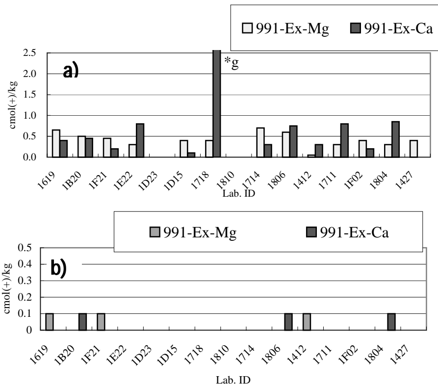
Figure 5.1. Laboratory average a) and range b) of Ex-Mg and Ca for No.991
